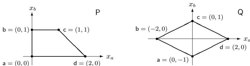
Fig. 1. Polytopes with different automorphism groups.
