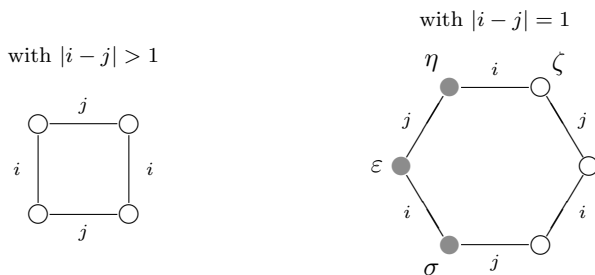
Fig. 2. A square and a hexagon in the permutohedral graph.
