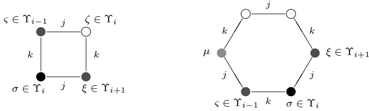
Fig. 3. The illustration of the proof of Lemma 4.8.
