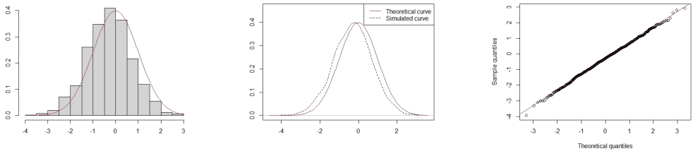
Fig. 5. The obtained results for \hat{f}_n(x) in model II.
