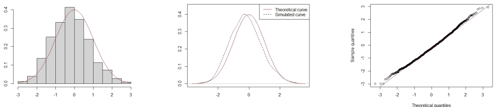
Fig. 7. The obtained results for \hat{\lambda}_n(x) in model II.
