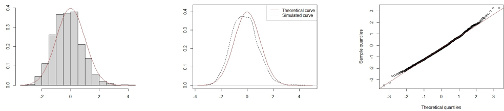
Fig. 9. The obtained results for \lambda_n^*(x) in model II.
