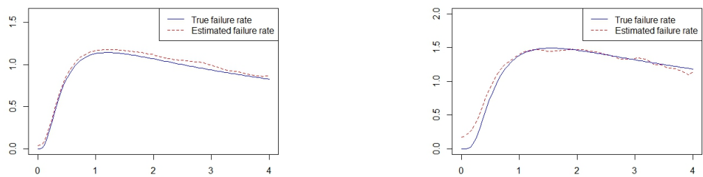
Fig. 3. Representation of \lambda_n^*(x) for model I (left graph) and model II (right graph).
