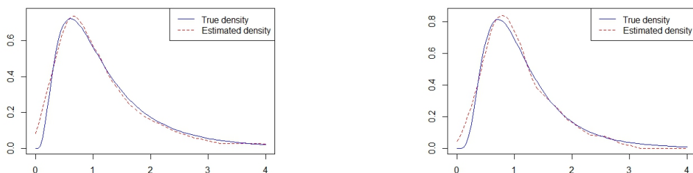
Fig. 1. Representation of \hat{f}_n(x) for model I (left graph) and model II (right graph).
