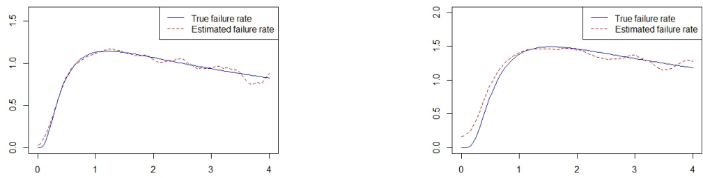
Fig. 2. Representation of \hat{\lambda}_n(x) for model I (left graph) and model II (right graph).
