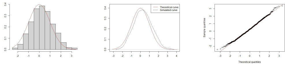
Fig. 4. The obtained results for \hat{f}_n(x) in model I.
