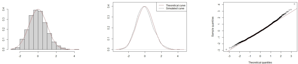
Fig. 6. The obtained results for \hat{\lambda}_n(x) in model I.
