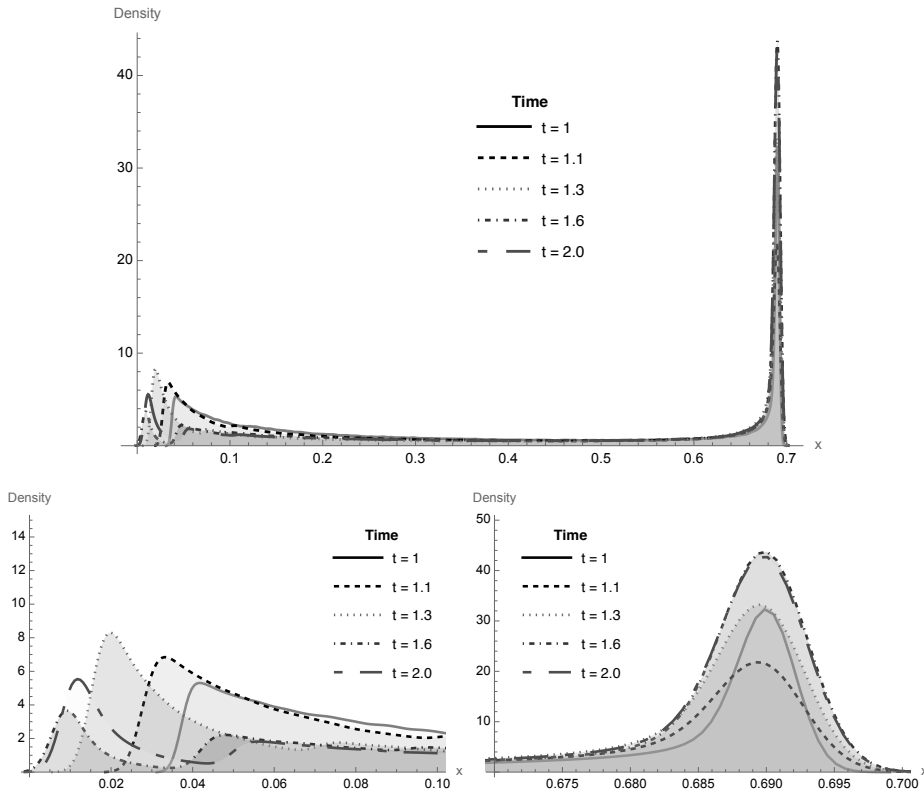
Fig. 7: Top: 1-PDF of the solution stochastic process X_A(t; H) given in (16) at the time instants t = \{1, 1.1, 1.3, 1.6, 2\} with a light/dark ratio r = 0.5 . The curves illustrate the evolution and the propagation of uncertainty induced by the random cycle period H . Bottom: Detail of the tails of the X_A(t; H) 1-PDF. The probability accumulation evidences the sensitivity of the system to extreme realizations of the random cycle period H .
