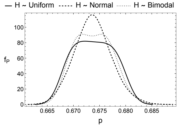
Fig. 6: PDF of P when H is distributed as described by (1)–(3).
