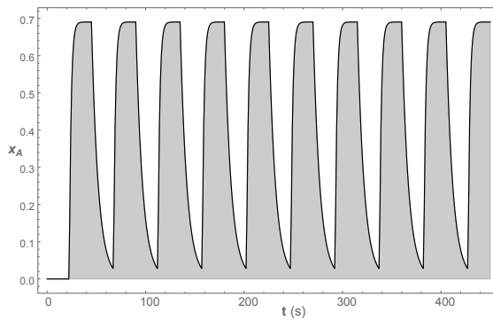
Fig. 2: Numerical solution of x_A(t; r) as given in Eq. (7), using a light cycle period of h = 45 s, irradiance levels I_a = 0 \mu\text{mol photons}^{-1} \text{m}^{-2} \text{s}^{-1} (dark phase) and I_b = 220 \mu\text{mol photons}^{-1} \text{m}^{-2} \text{s}^{-1} (light phase), with a light/dark ratio of r = 0.5 . Model parameters are taken from [25].
