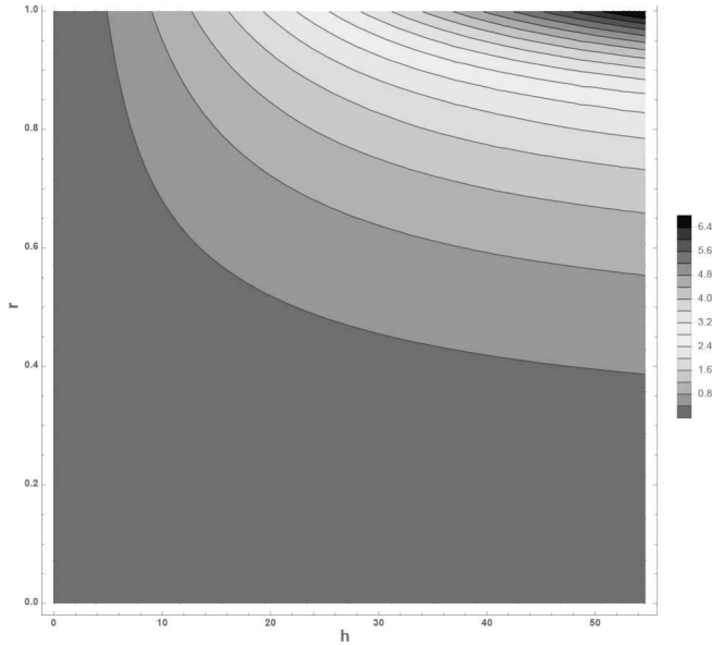
Fig. 3: Contour plots of the elasticity E_h (10) as h and r change: h \in (0, e^4) , r \in (0, 1) , using irradiance levels I_a = 0 \mu\text{mol photons}^{-1} \text{m}^{-2} \text{s}^{-1} (dark phase) and I_b = 220 \mu\text{mol photons}^{-1} \text{m}^{-2} \text{s}^{-1} (light phase). Model parameters and experimental data are taken from [25].
