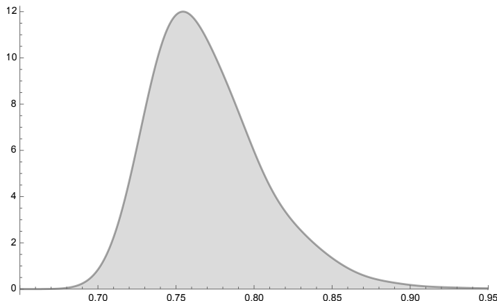
Fig. 8: PDF of the productivity P , given by (25) and (28), computed in the quasi-steady state regime using K = 3 averaging cycles and a light/dark ratio r = 0.5 .
