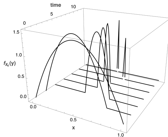
Fig. 4: PDF of the transferred initial condition f_{X_0} evaluated at y = xg_1(t, h) - g_2(t, h) for x \in [\varepsilon, 1 - \varepsilon] \subset (0, 1) with \varepsilon = 0.001 and times t = 1, \dots, 10 with \alpha = \beta = 2 , h = 5 , and r = 0.5 . All other model parameters as described in Table 1. The plot illustrates the progressive concentration of the probabilistic density as time increases tending to a leptokurtic shape.
