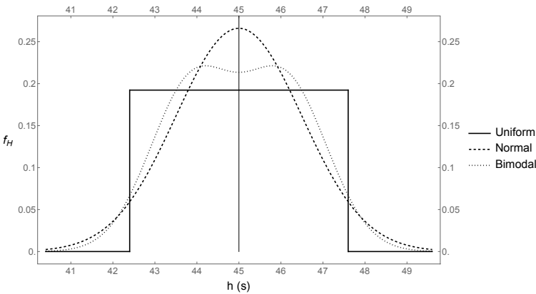
Fig. 5: Probability density functions (1)–(3) of H as defined in Table 2.
