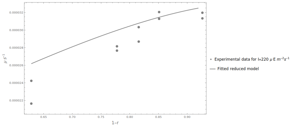
Fig. 1: Plot of \mu as defined in Eq. (8), using a light cycle period of h = 45 s, irradiance levels I_a = 0 \mu\text{mol photons m}^{-2}\text{s}^{-1} (dark phase) and I_b = 220 \mu\text{mol photons m}^{-2}\text{s}^{-1} (light phase). Model parameters and experimental data are taken from [25].
