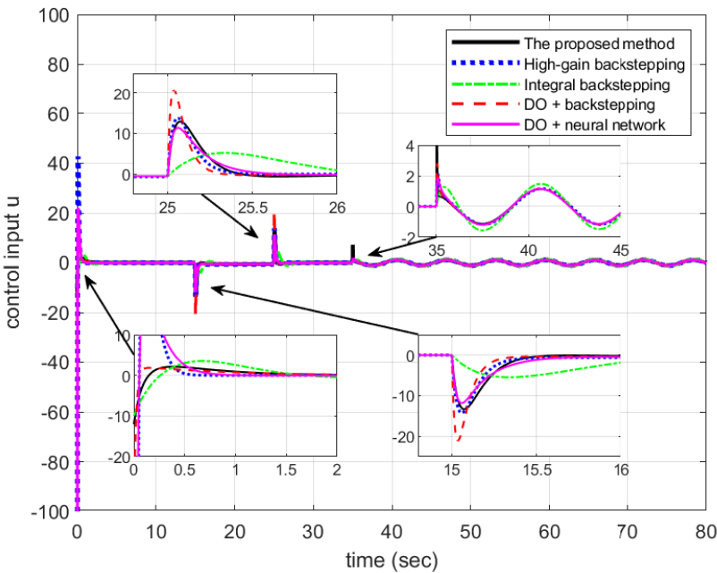
Fig. 1. Input trajectories for numerical simulation (53) under the proposed (black solid), disturbance observer-backstepping (red dashed), high-gain backstepping (blue dotted), neural network-based composite anti-disturbance control (magenta solid) and integral backstepping (green dash-dotted) methods.
