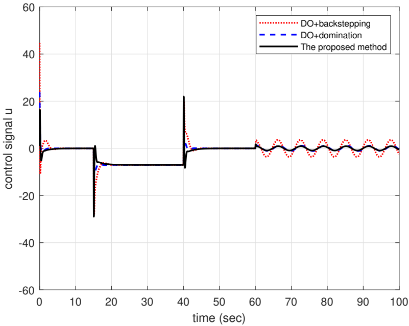
Fig. 3. Input trajectories of application simulation (54) under the three controllers. The responses of the proposed method, disturbance observer-backstepping method, and homogeneous dominance-based disturbance observer control are depicted as black solid, red dotted and blue dashed lines, respectively.
