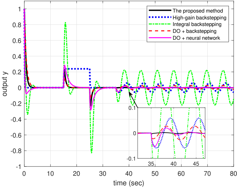
Fig. 2. Output trajectories for numerical simulation (53) under the proposed (black solid), disturbance observer-backstepping (red dashed), high-gain backstepping (blue dotted), neural network-based composite anti-disturbance control (magenta solid) and integral backstepping (green dash-dotted) methods.
