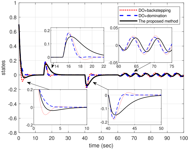
Fig. 4. State trajectories of application simulation (54) under the three controllers. The responses of the proposed method, disturbance observer-backstepping method, and homogeneous dominance-based disturbance observer control are depicted as black solid, red dotted and blue dashed lines, respectively.
