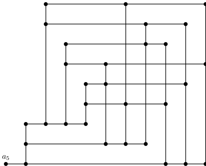
Fig. 2. The Greechie diagram of an orthomodular lattice representing a counterexample.
