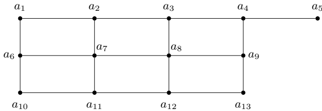
Fig. 1. The Greechie diagram of an orthomodular poset representing a counterexample.
