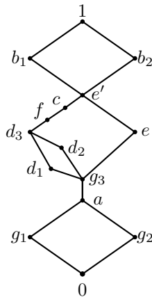
Fig. 8. The lattice L_7 in Example 3.10 (vii)
