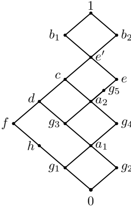
Fig. 5. The lattice L_4 in Example 3.10 (iv)
