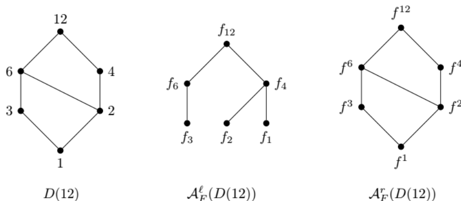
Fig. 7. The Hasse diagrams of the lattices (D(12), |, gcd, lcm) , (\mathcal{A}_F^r(D(12)), \leq^r, \wedge^r, \vee^r) , and the poset (\mathcal{A}_F^\ell(D(12)), \leq^\ell) .
