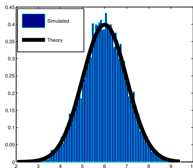
Fig. 3: pdf of \hat{z}_5 for singular W .
