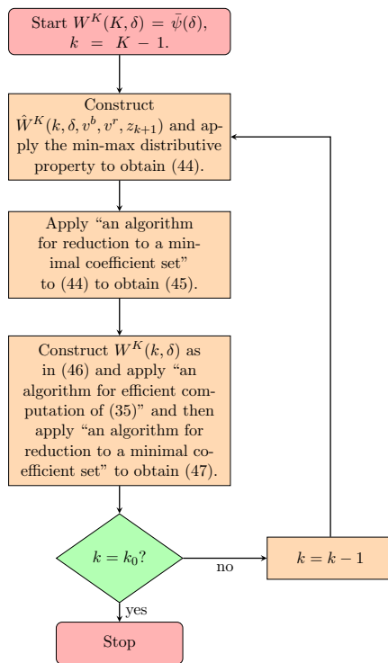
Fig. 8. Computation of solution.
