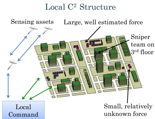
Fig. 2. Example physical region.
