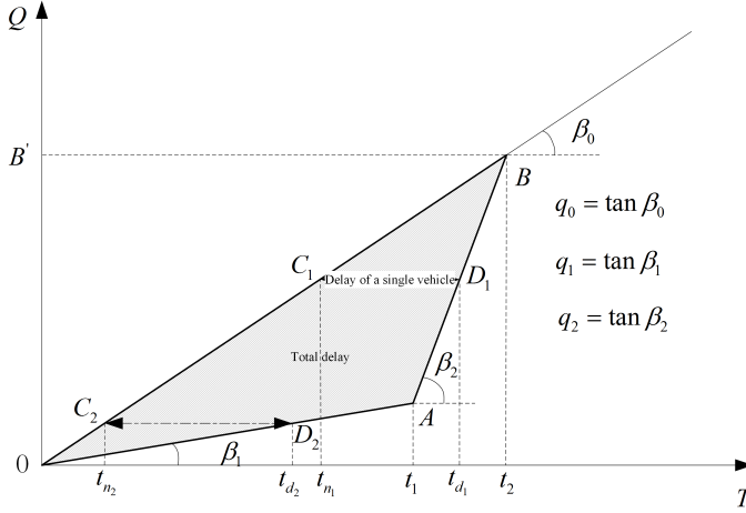
Fig. 7. Calculation of total delay time.
