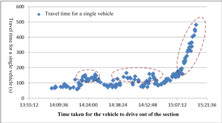
Fig. 3. Vehicle travel time data related to traffic incident.
