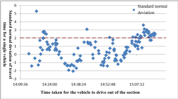
Fig. 4. SND data of single vehicle travel time which related to common traffic incidents.
