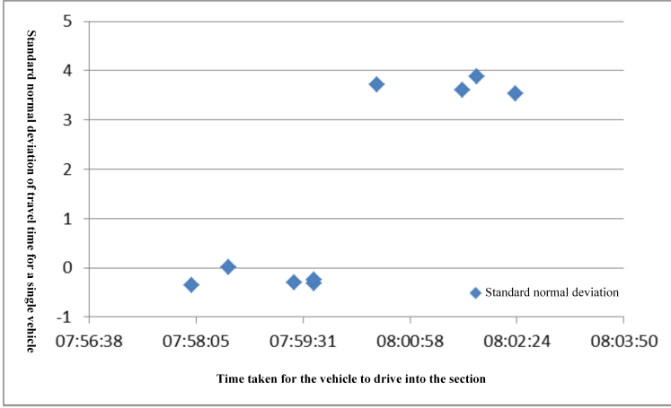
Fig. 6. SND data of single vehicle travel time which related to a serious traffic incident.
