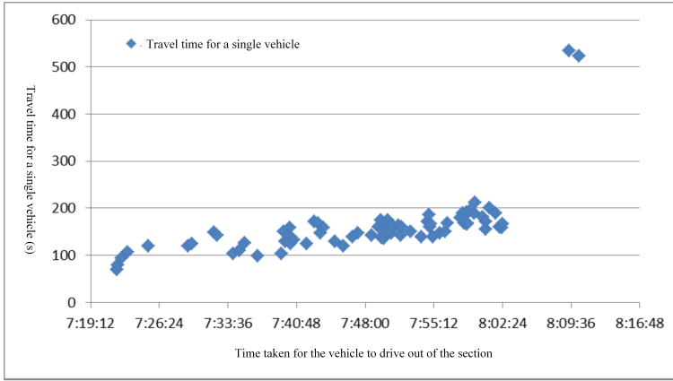
Fig. 5. Vehicle travel time data related to a serious traffic accident.
