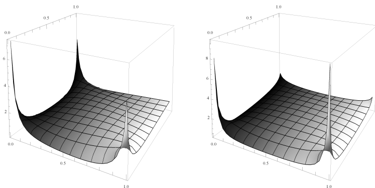
Fig. 6. 3D plot of the density functions for the optimal models (4C – left, 4B – right) of the relation between the daily returns of N. Y. stock index and gold for the time period 20. 7. 2007 – 4. 3. 2009.
