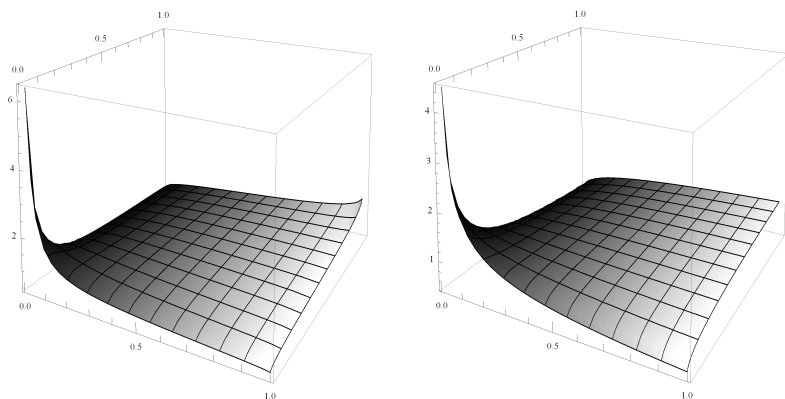
Fig. 8. 3D plot of the density functions for the optimal models ( 5F – left, 5G – right) of the relation between the daily returns of N. Y. stock index and gold for the time period 5. 3. 2009 – 3. 12. 2010.
