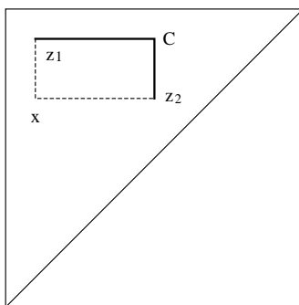
Fig. 2. Forbidden separation.
