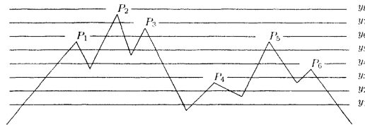
Fig. 2. The analyzed unipolar waveform.
