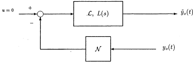
Fig. 2. Open loop path for distortion definition.
