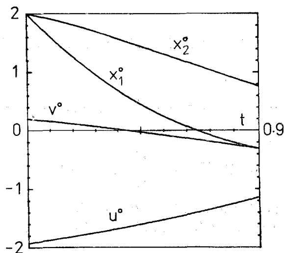
Fig. 1. Optimal solution of Example 1.
