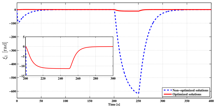
Fig. 6. Variation diagram of compensation vector \xi_1 .
