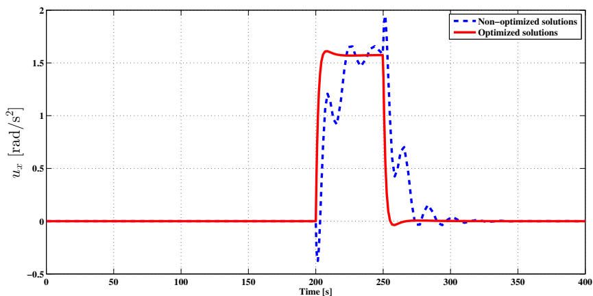
Fig. 8. Variation diagram of control signal u_x .
