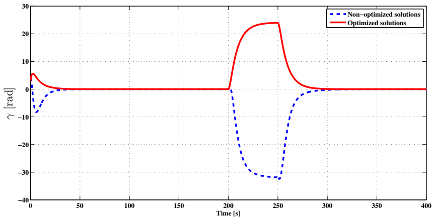
Fig. 3. Variation diagram of yaw angle \gamma .
