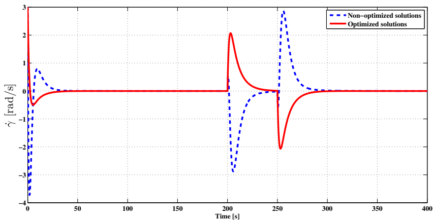
Fig. 5. Variation diagram of yaw angular velocity \dot{\gamma} .
