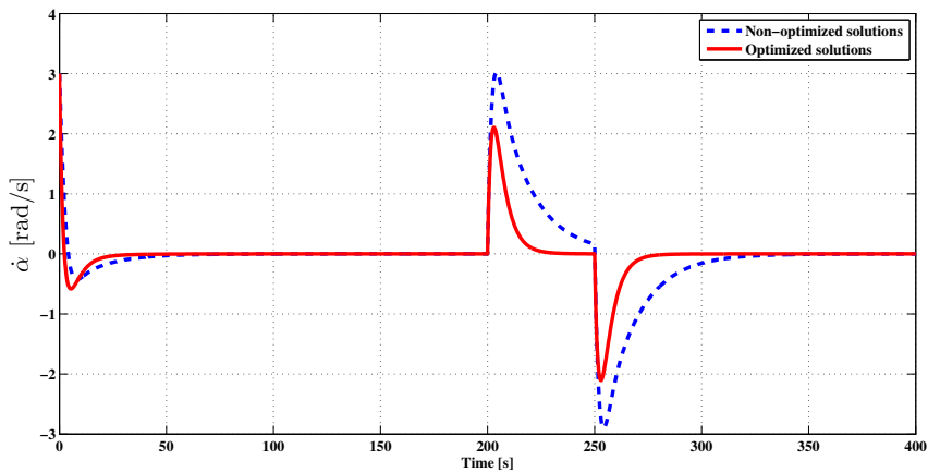
Fig. 4. Variation diagram of roll angular velocity \dot{\alpha} .
