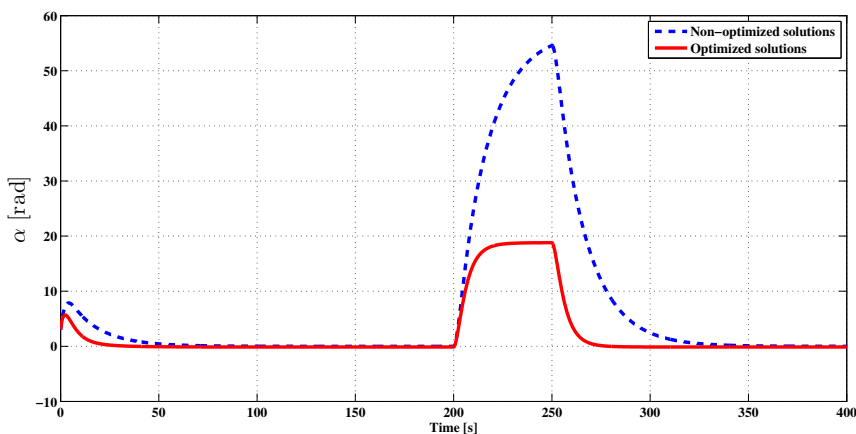
Fig. 2. Variation diagram of roll angle \alpha .
