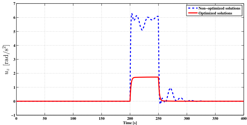
Fig. 9. Variation diagram of control signal u_z .
