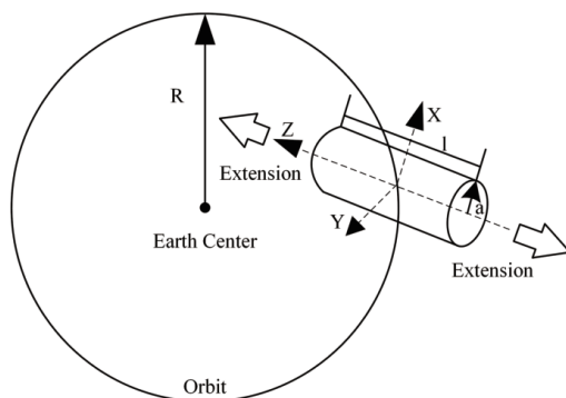
Fig. 1. Coordinate systems.
