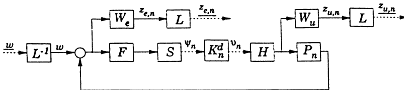
Fig. 9. Sampled-data feedback loop input/output lifting.
