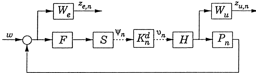
Fig. 4. Purely finite-dimensional sampled-data feedback loop.
