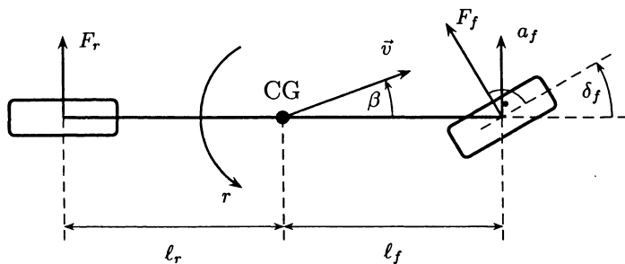
Fig. 7. Single-track model.
