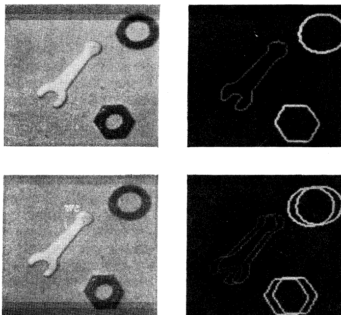
Fig. 5. Example of moving object recognition, using preprocessing digital filtering and boundary FFT matching: two consecutive frames are shown with input digitized images at the left and recognized objects at the right (each object is recognized with different colour, here appearing as a different gray-level).
