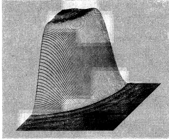
Fig. 1. Example of spatial frequency response (amplitude in one quadrant) of a circular 2-D FIR low-pass digital filter ( 16 \times 16 coefficients).
