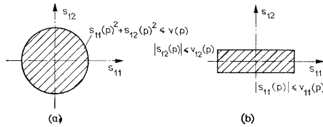
Fig. 3. Set of matrices S_2 = (s_{11} \ s_{12}) for SS 2 with \dim z = 2 , \dim s = 1 .
